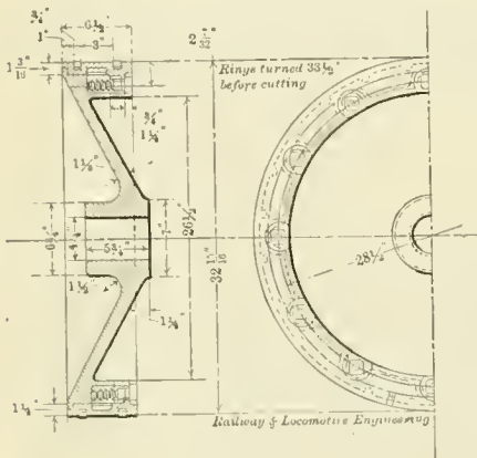
LOW-PRESSURE PISTON OF ROGERS COMPOUND.
